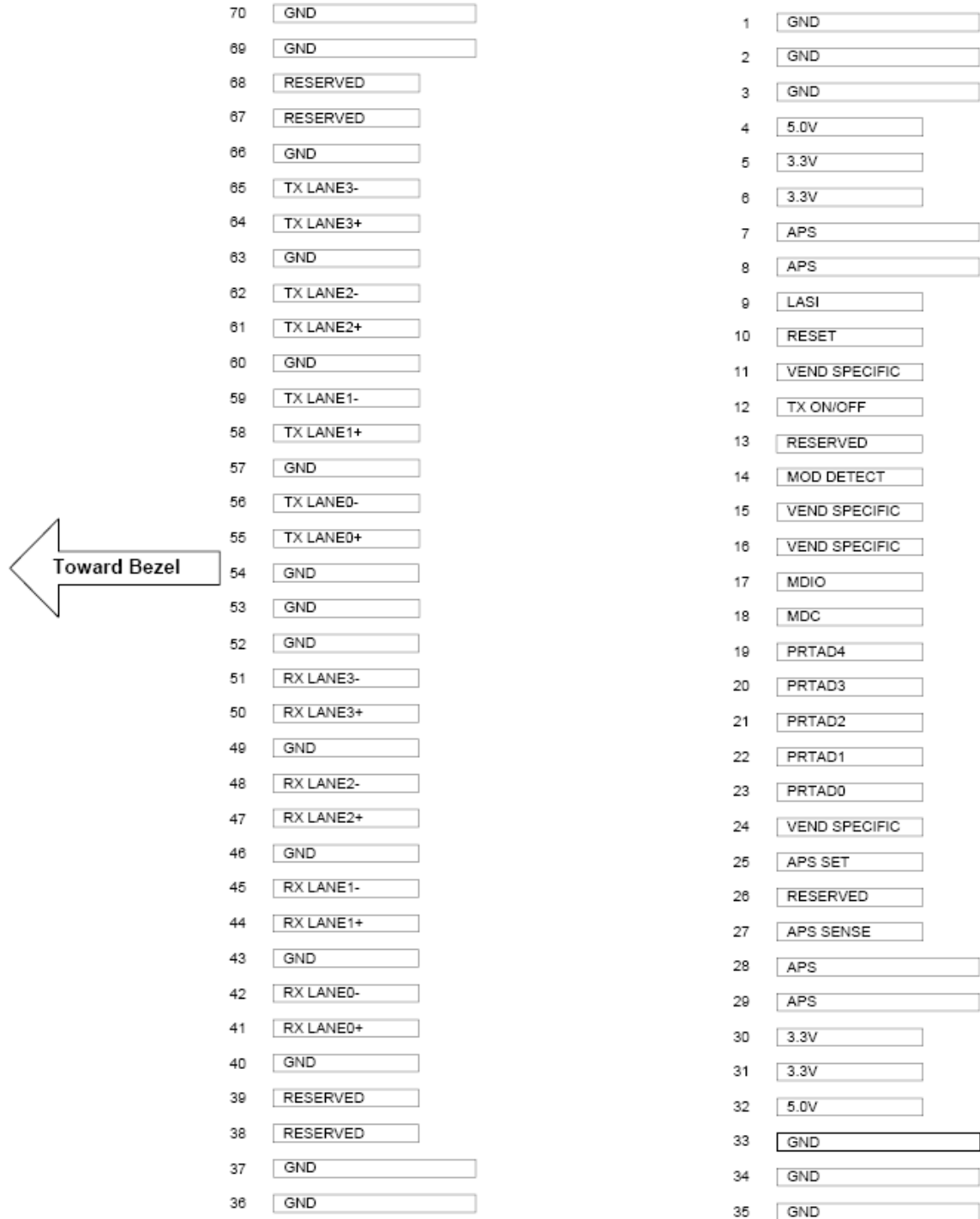
Figure2.Electrical Pin-out Details
